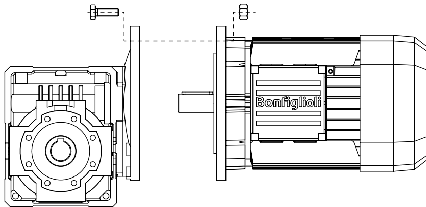
B5 - Motor Mounting Large Flange (for Motor with Through Holes)
